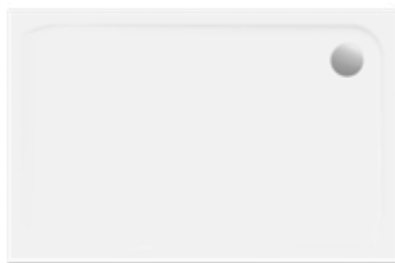
DIANA S100 Acryl-Rechteck-Brausewanne superflach, Tiefe 35 mm, Ablaufloch 90 mm, weiß, 900 x 750 mm, (DI224101001) 252,- € 900 x 800 mm, (DI224102001) 308,- € 1000 x 800 mm, (DI224105001) 350,- € 1200 x 800 mm, (DI224106001) 404,- € 1200 x 900 mm, (DI224107001) 428,- € 1400 x 900 mm, (DI224108001) 457,- €
